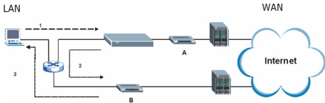
Figure 391 “Triangle Route” Problem
