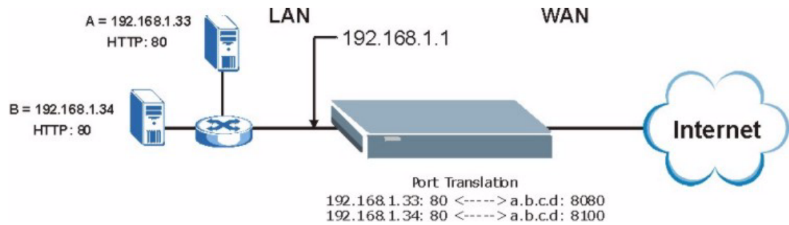
Figure 145 Port Translation Example
