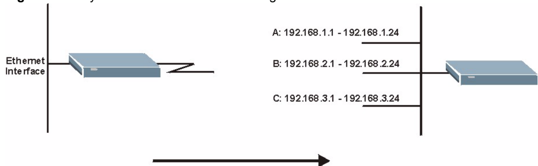
Figure 25 Physical Network & Partitioned Logical Networks
