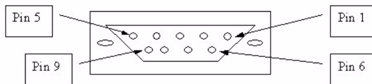
Figure 362 Console/Dial Backup Port Pin Layout
