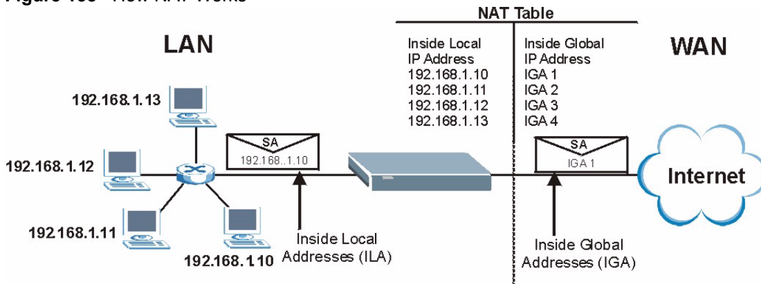
Figure 138 How NAT Works
