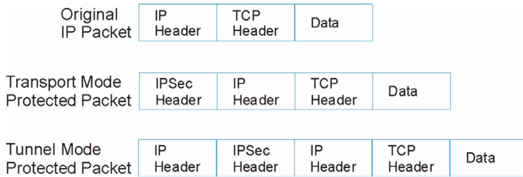
Figure 106 Transport and Tunnel Mode IPSec Encapsulation
