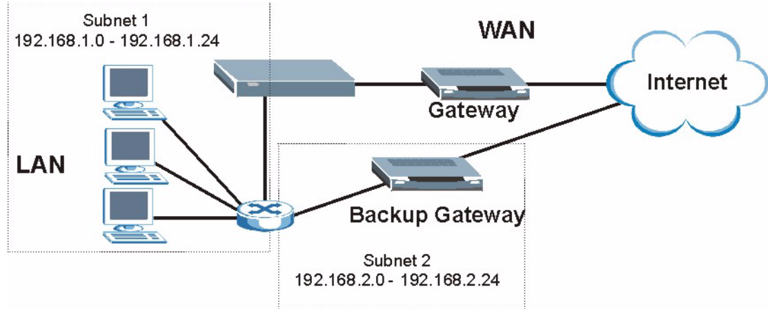
Figure 53 Traffic Redirect LAN Setup
