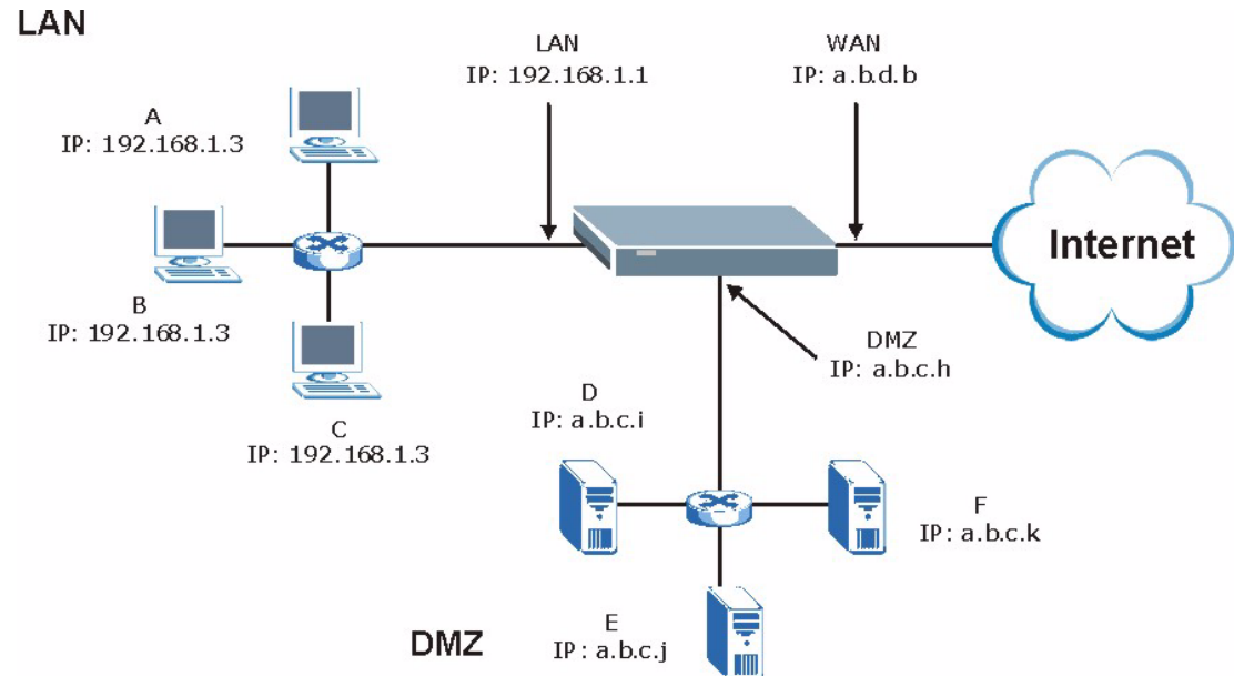
Figure 59 DMZ Public Address Example
