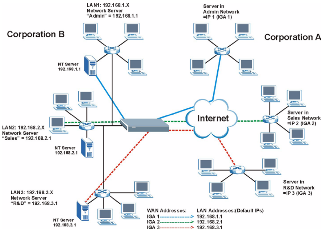
Figure 139 NAT Application With IP Alias
