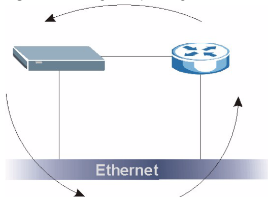
Figure 27 Bridge Loop: Bridge Connected to Wired LAN
