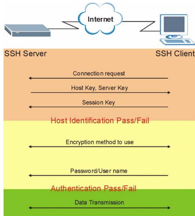
Figure 178 How SSH Works
