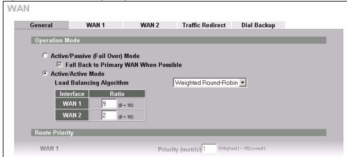
Figure 47 Load Balancing: Weighted Round Robin
