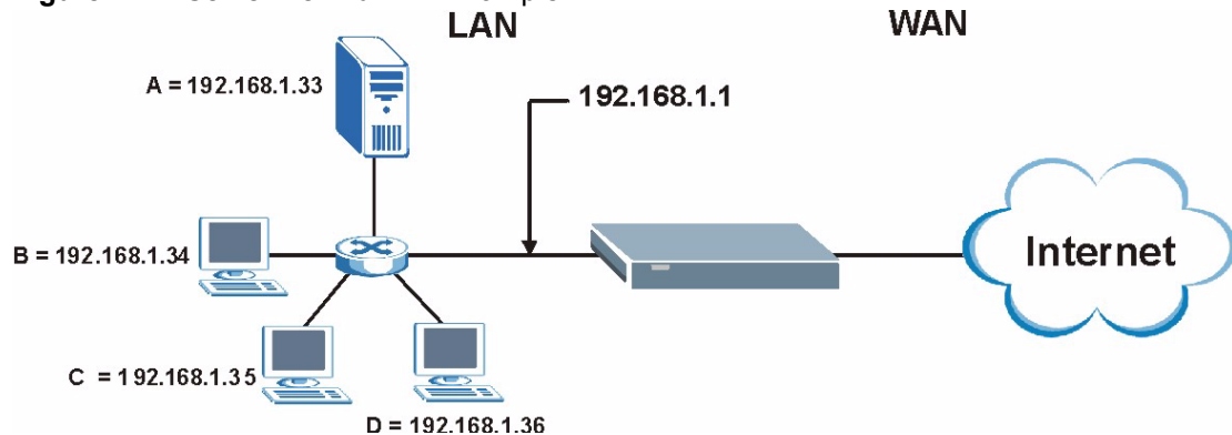
Figure 274 Server Behind NAT Example
