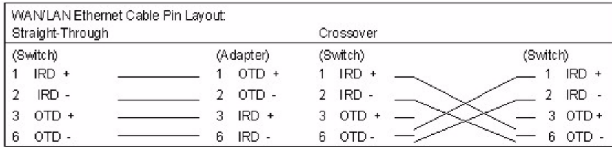
Figure 363 Ethernet Cable Pin Assignments
