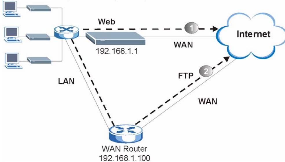
Figure 346 Example of IP Policy Routing
