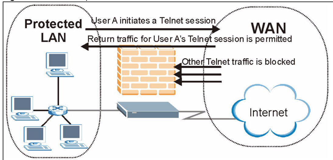
Figure 50 Stateful Inspection
