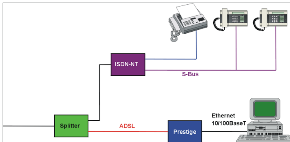
Figure 260 Prestige with ISDN
