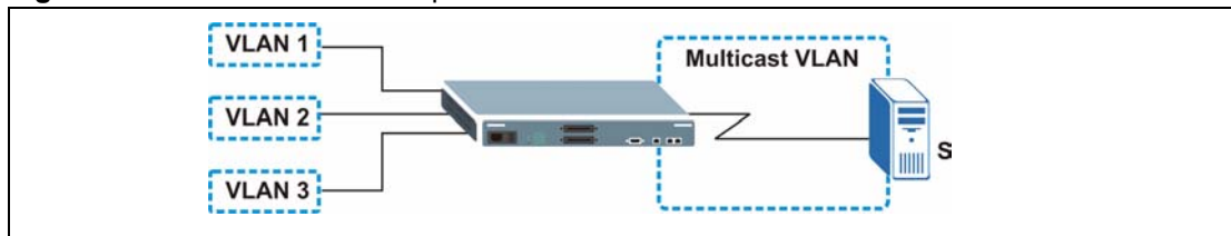
Figure 61 MVR Network Example
