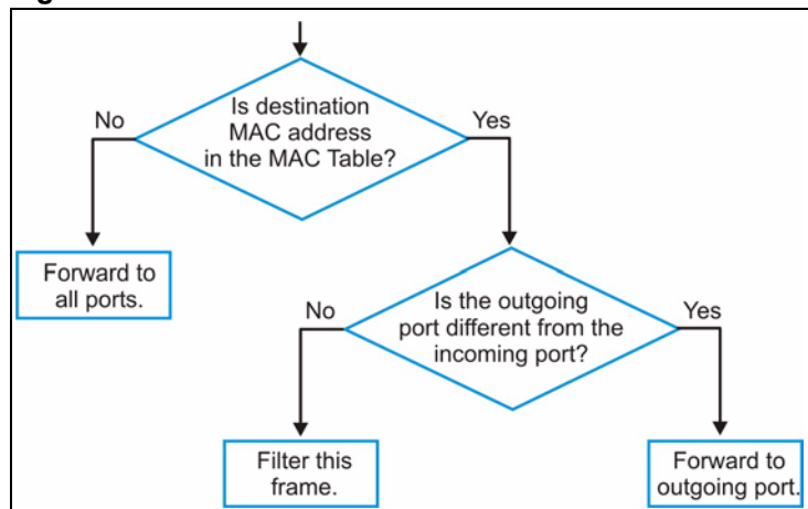
Figure 102 MAC Table Flowchart
