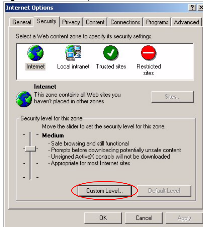
Figure 111 Internet Options
