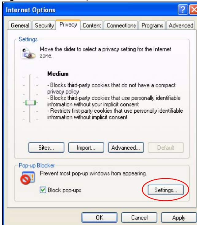
Figure 109 Internet Options
