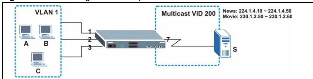
Figure 65 MVR Configuration Example
