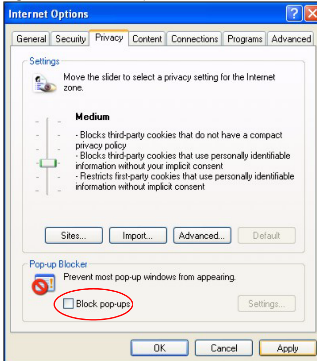
Figure 108 Internet Options
