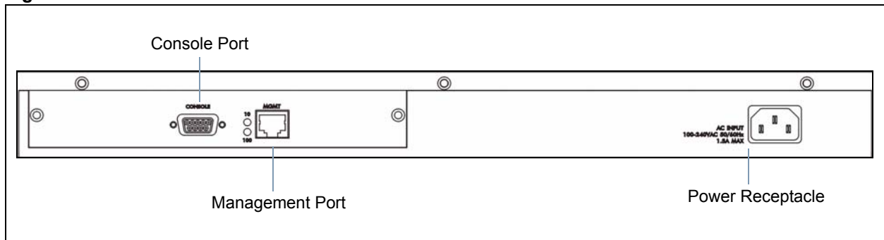
Figure 10 Rear Panel
