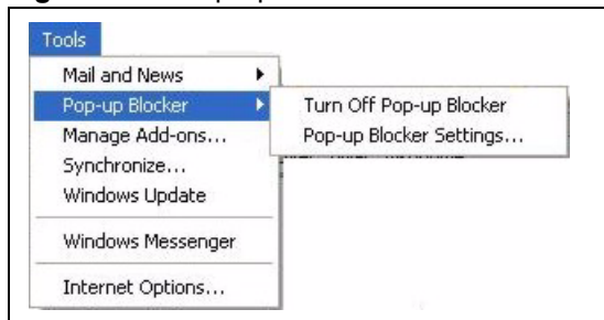
Figure 107 Pop-up Blocker
