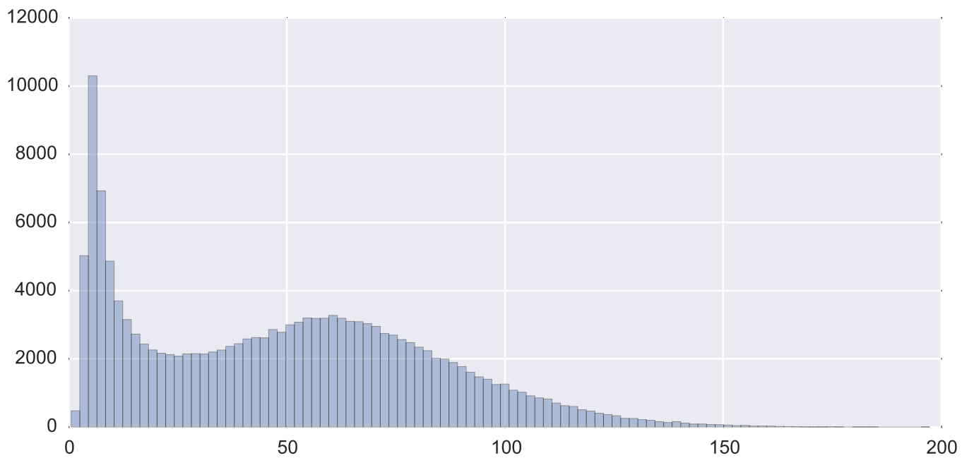
Subject 27951 tSNR inside the mask
