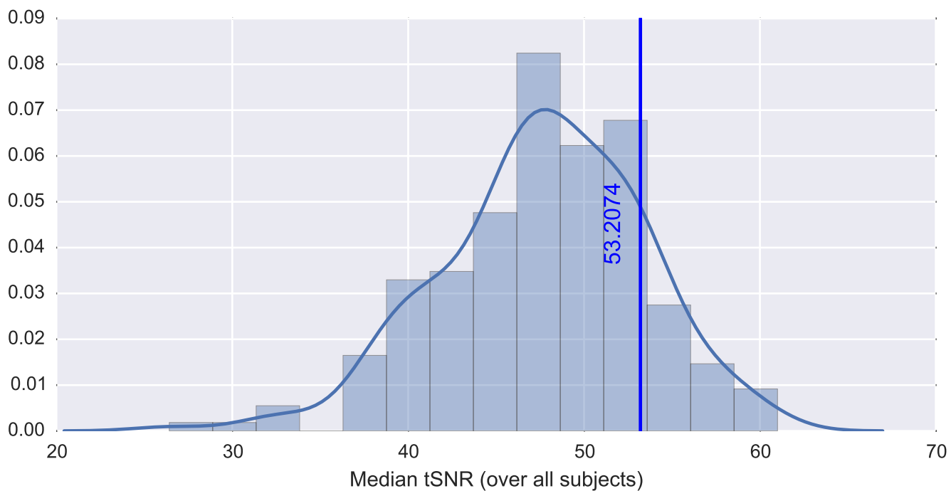
Subject 27614 tSNR inside the mask
