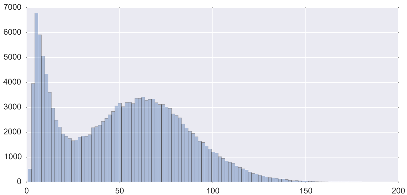
Subject 27614 tSNR inside the mask
