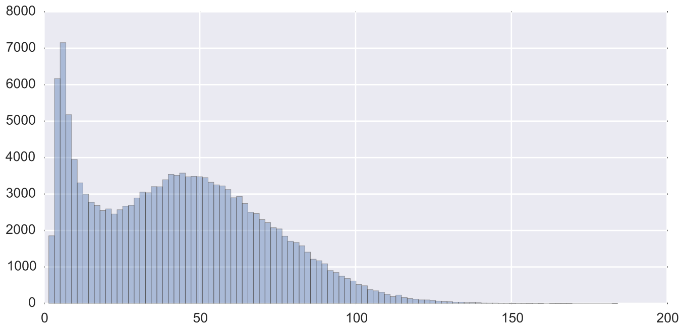
Subject 23860 tSNR inside the mask
