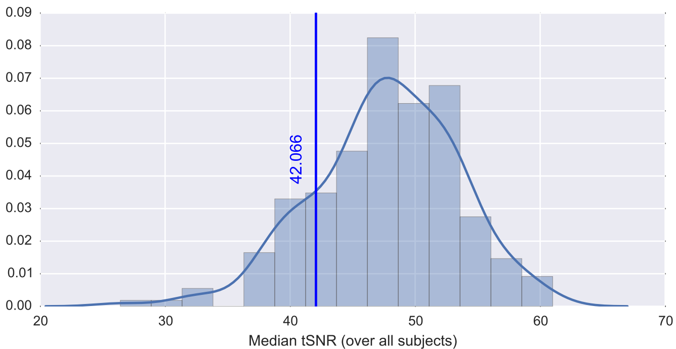
Subject 23860 tSNR inside the mask
